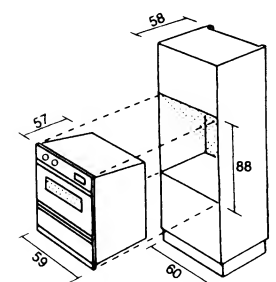
⑦ Built-in cooker
